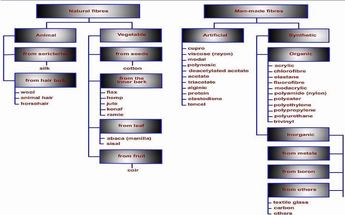
Classification of fibres
